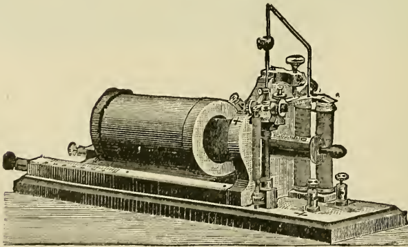
FIG. 112. — Sledge Induction coil.
